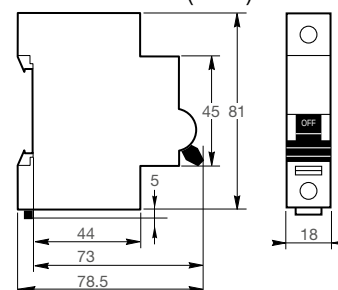
Dimensions (mm)
