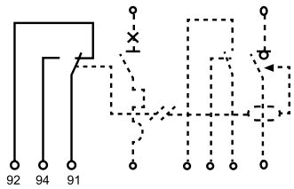
A9N26927 - SD fault finding switch
